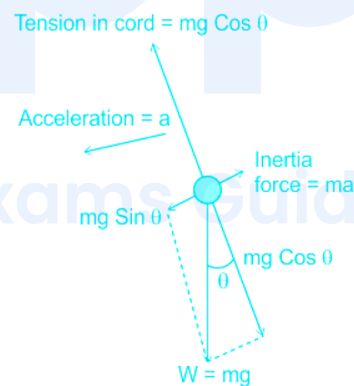
(b) Forces acting on bob
