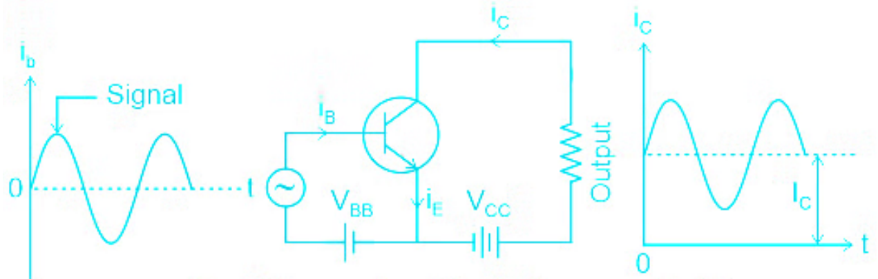
Transistor as Amplifier in Common Emitter
