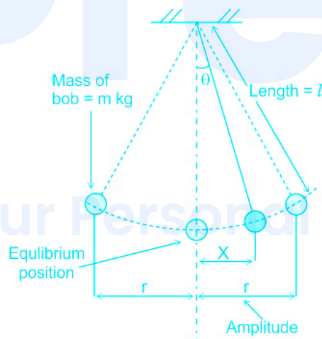
(a) Simple pendulum
