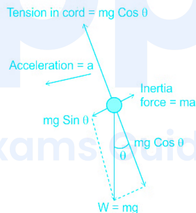
(b) Forces acting on bob
