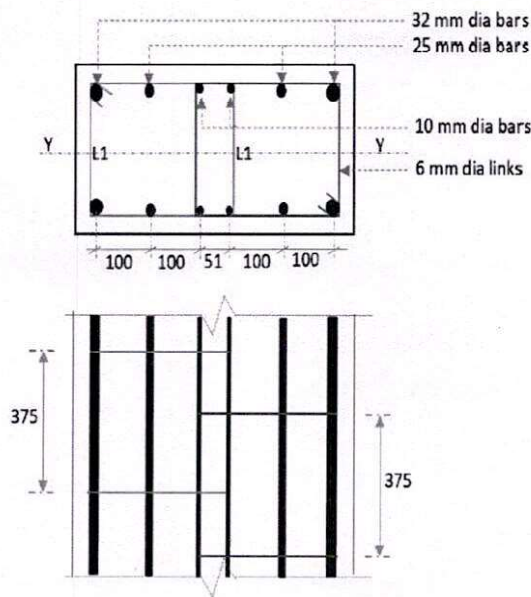
Figure (a): Cross-sectional view of an RC column. The longitudinal reinforcements are symmetrically placed. Bar diameters are given for both longitudinal and transverse reinforcements. Center to center distances between the bars along the longer edge are also mentioned.
